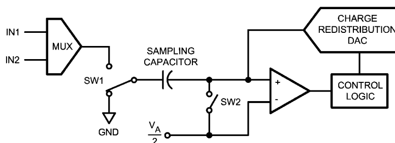
FIGURE 2. ADC082S051 in Hold Mode
