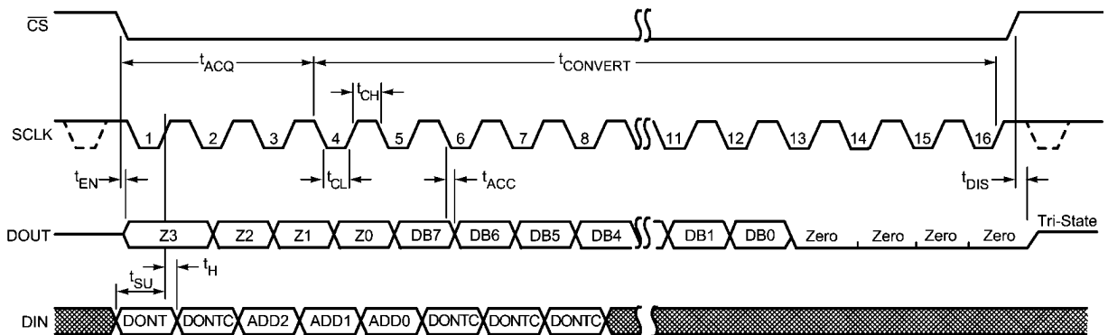
ADC082S051 Serial Timing Diagram
