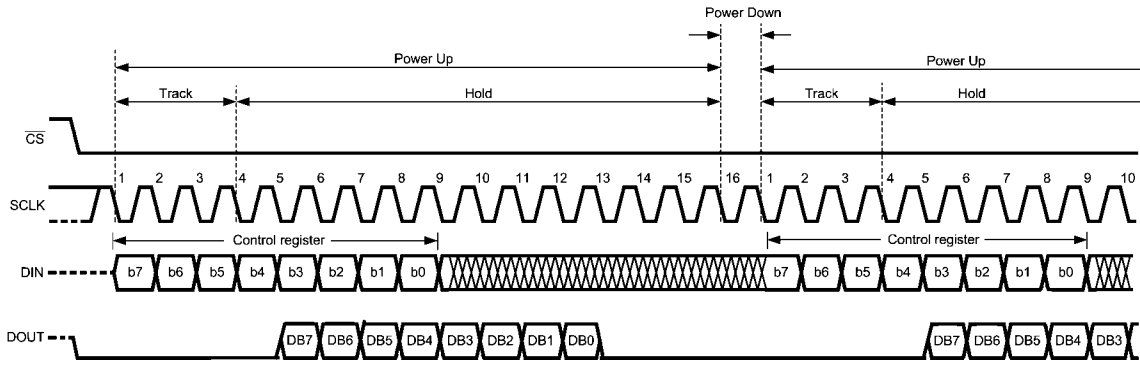
ADC082S051 Operational Timing Diagram
